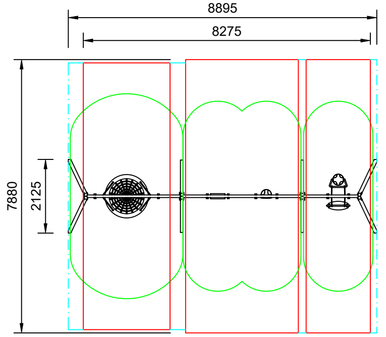
Plan View Scale: 1:110
