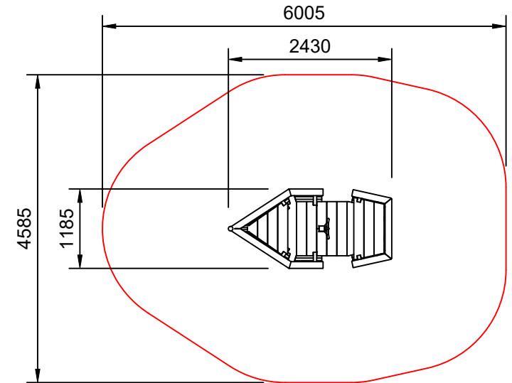
Plan View Scale: 1:80
