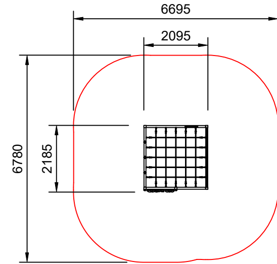
Plan View Scale: 1:125
