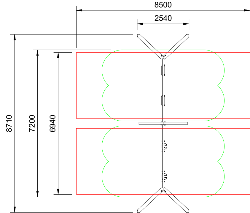
Plan View Scale: 1:110
